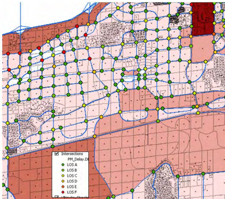
Figure 21. Intersection LOS in GIS format, West Des Moines, IA
